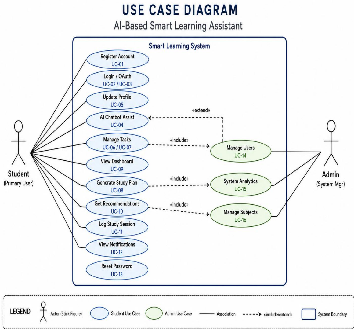
Figure: Use Case Diagram of the AI-Based Smart Learning Assistant
